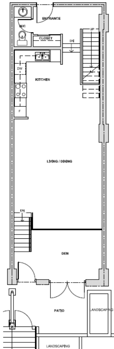
LEVEL 1: 776 SQFT
